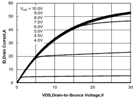
Output Characteristics
