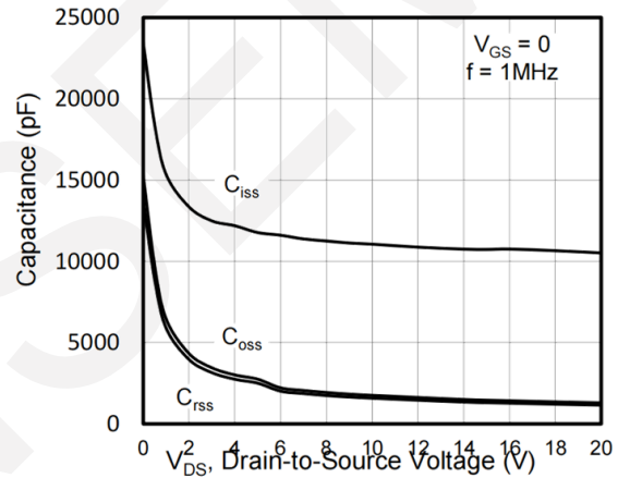
Capacitance
