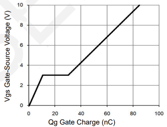
Gate Charge
