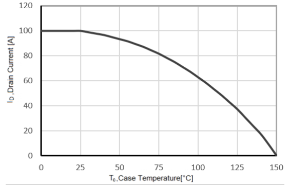
Drain current vs. Case Temperature
