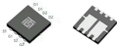
PDFN3X3 Pin Description
