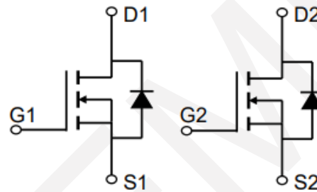
Schematic Diagram
