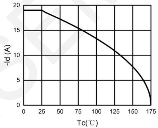
ID Current Derating
