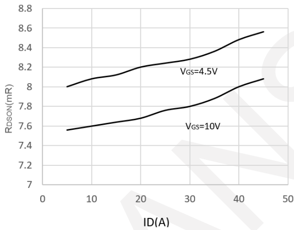
Rdson-Drain Current
