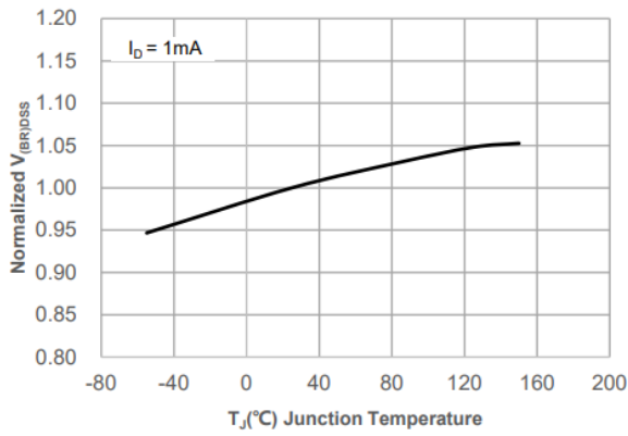
V_{DSS} vs Junction Temperature
