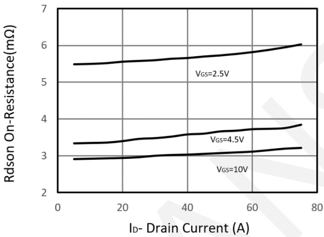
Rdson-Drain Current
