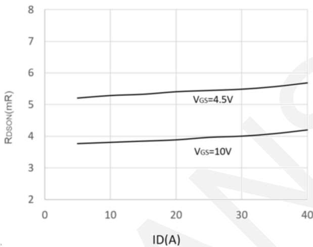
Rdson-Drain Current
