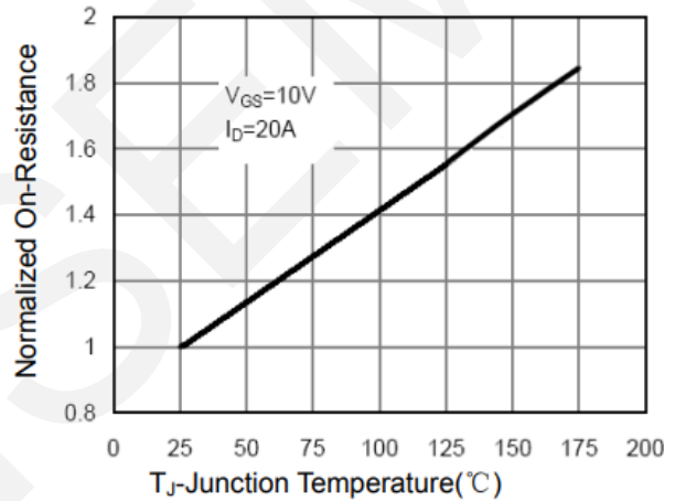
Rdson-Junction Temperature
