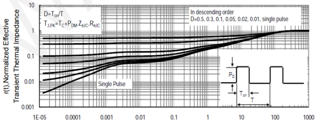
Square Wave Pulse Duration(sec) Normalized Maximum Transient Thermal Impedance
