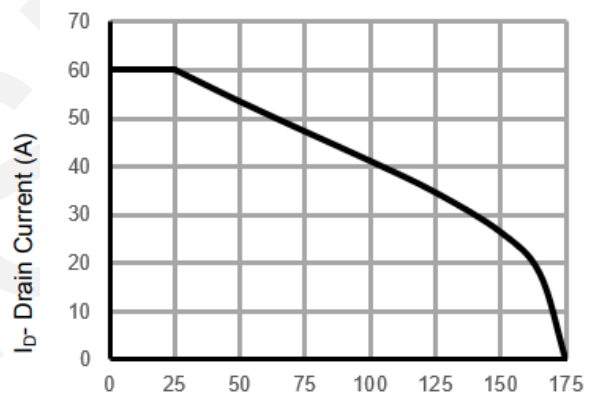
T J -Junction Temperature(°C) ID Current – Junction Temperature
