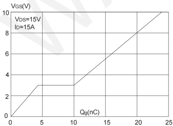
Gate Charge
