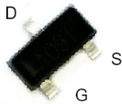
Pin Description SOT23
