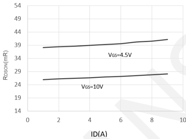
Drain-Source On-Resistance
