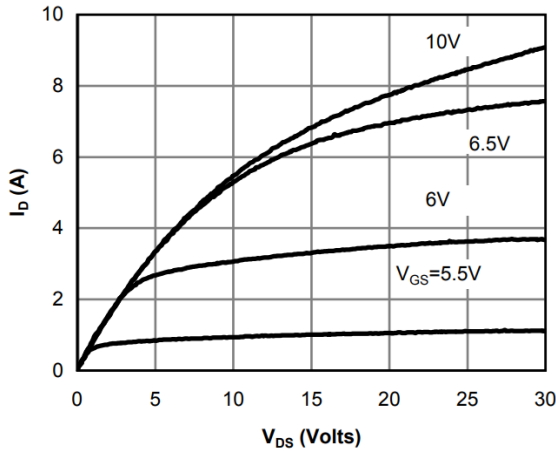
On-Region Characteristics
