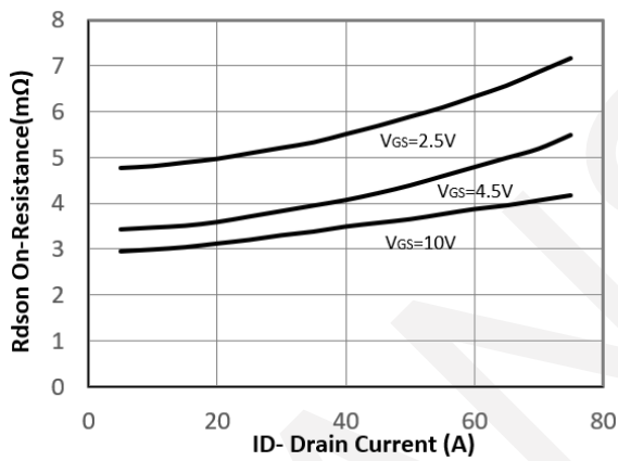
Rdson-Drain Current
