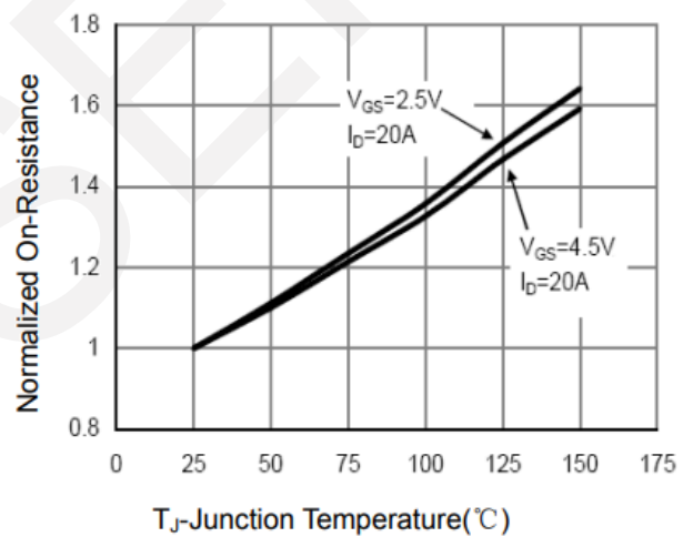
Rdson-Junction Temperature
