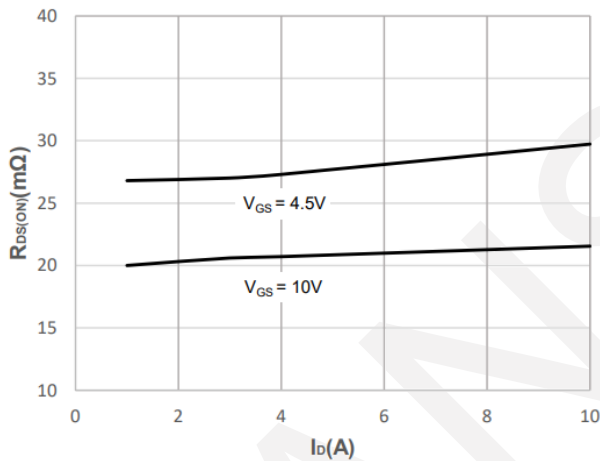
Drain-Source On-Resistance
