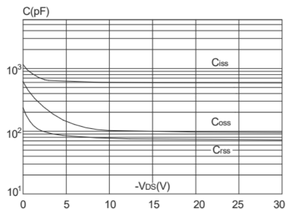
Capacitance Characteristics
