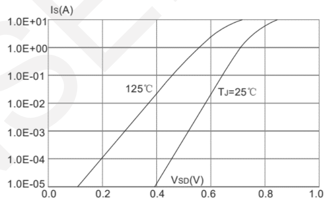
Body Diode Characteristics
