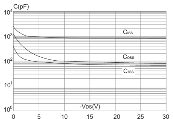
Capacitance Characteristics
