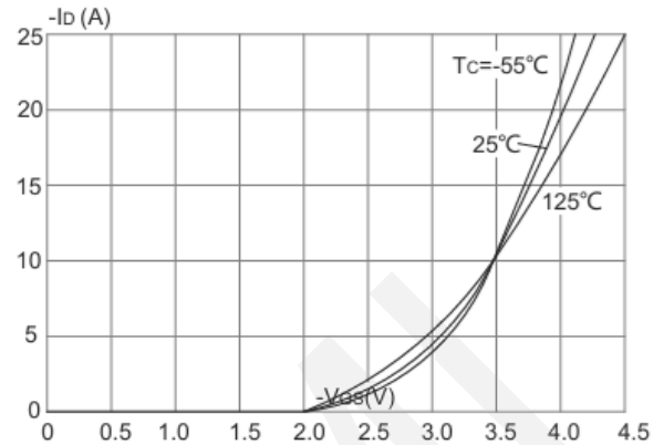
Transfer Characteristics
