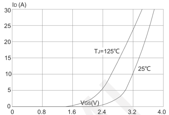
Transfer Characteristics
