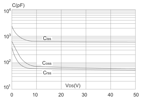
Capacitance Characteristics
