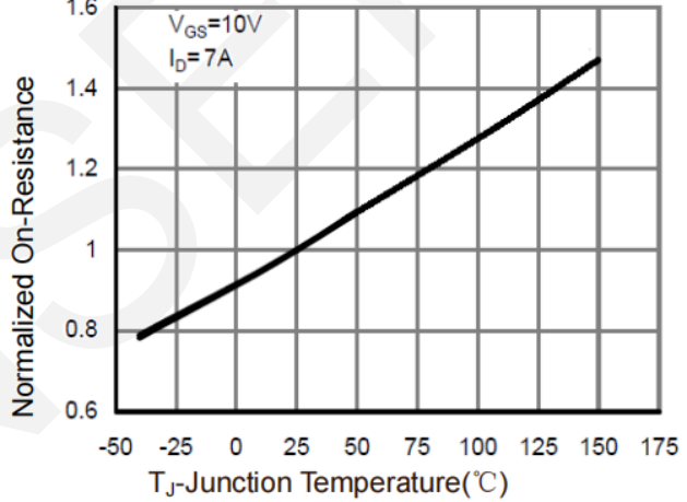
Rdson-Junction Temperature
