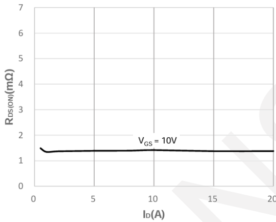
Rdson-Drain Current
