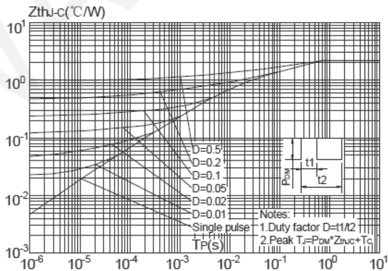
Maximum Effective Transient Thermal Impedance
