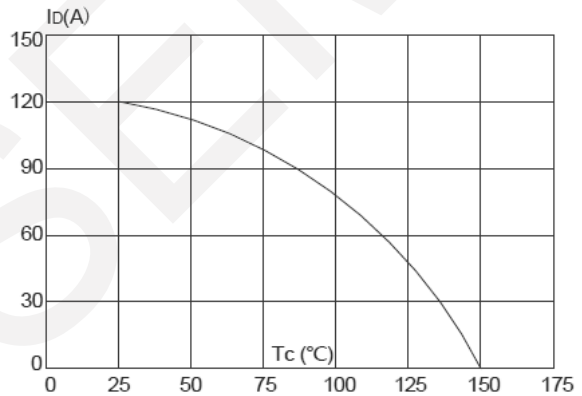
Continuous Drain Current vs. Case Temperature
