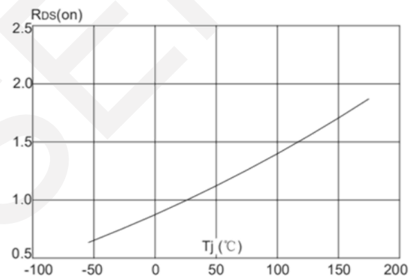
Rdson-Junction Temperature
