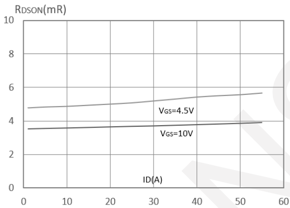
Rdson-Drain Current
