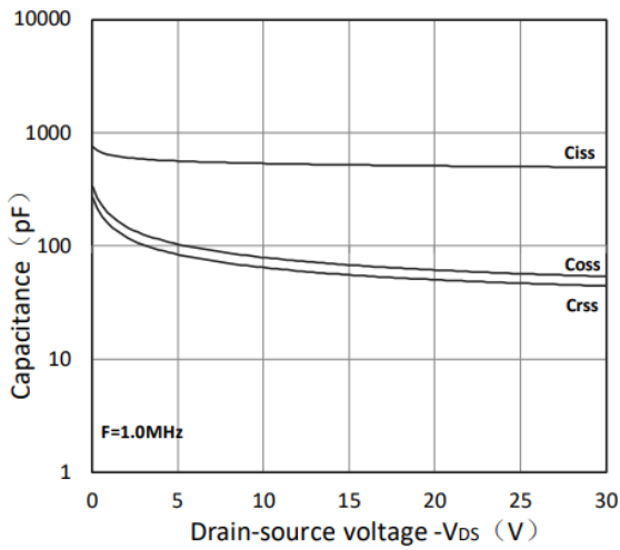
Capacitance Characteristics
