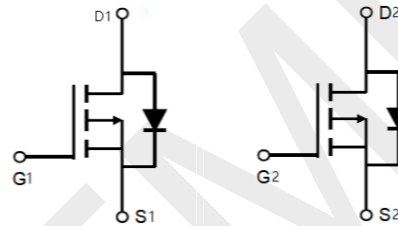
Schematic Diagram
