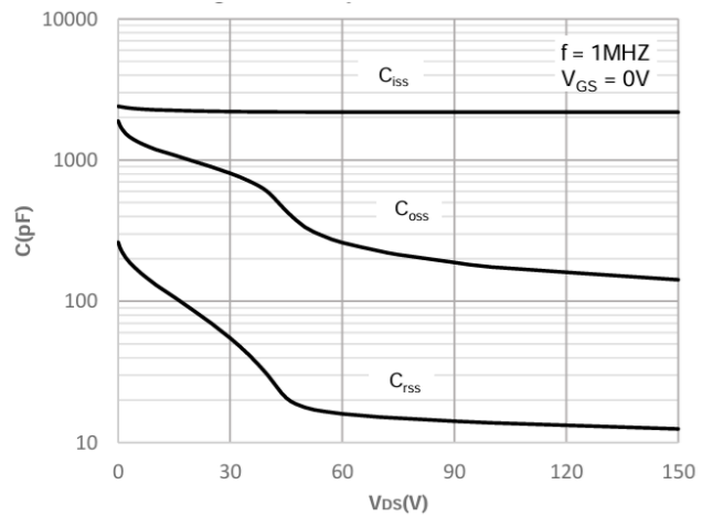
Capacitance Characteristics
