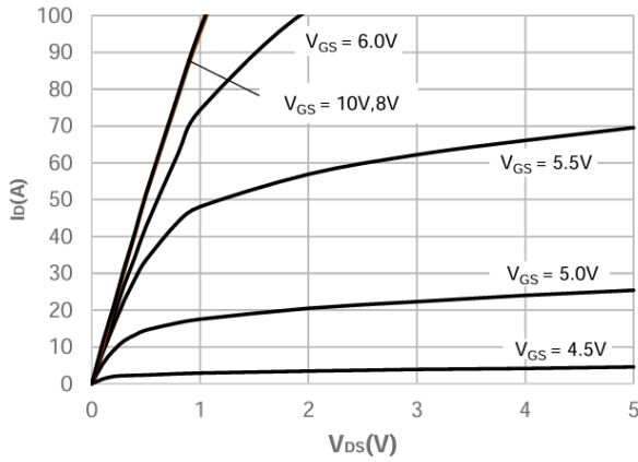
Saturation Characteristics
