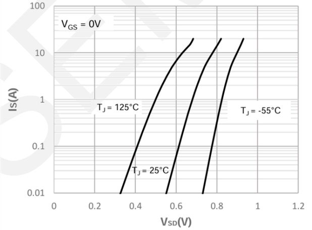
Body-Diode Characteristics
