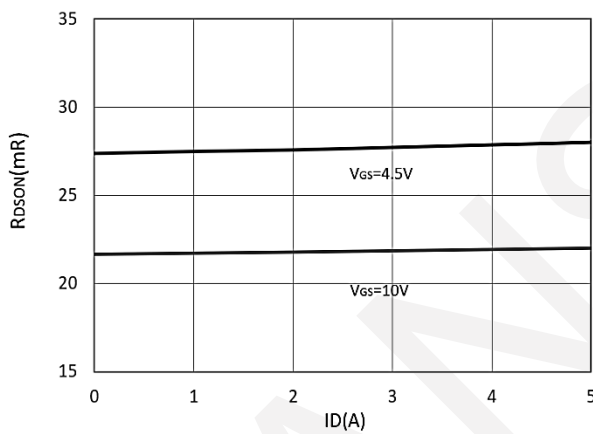
Drain-Source On-Resistance
