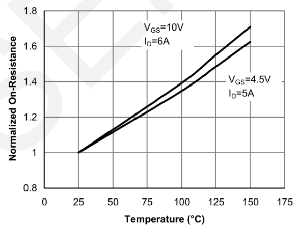
Drain-Source On-Resistance
