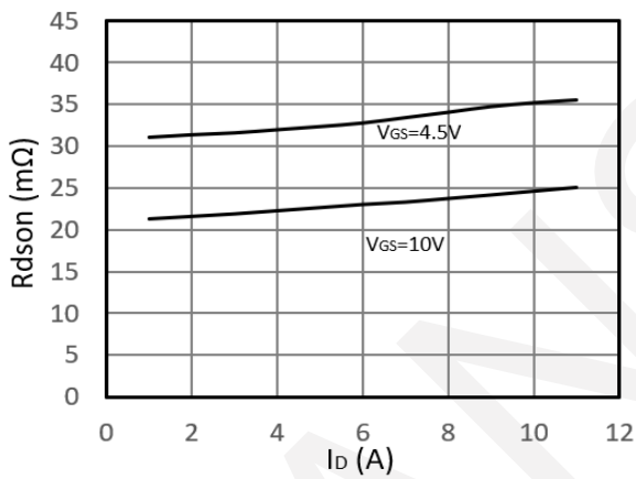
Drain-Source On-Resistance
