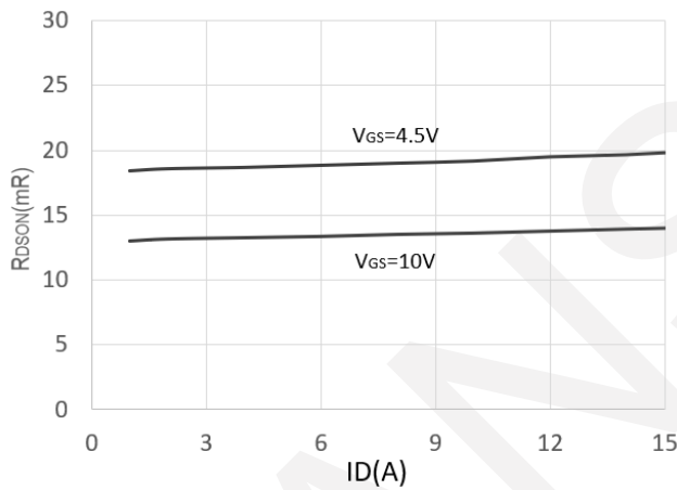
Drain-Source On-Resistance
