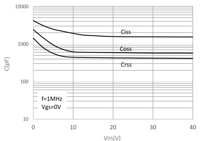
Capacitance Characteristics
