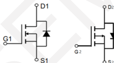
N-Channel P-Channel
