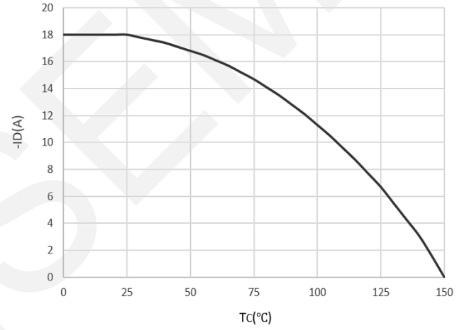
Current De-rating
