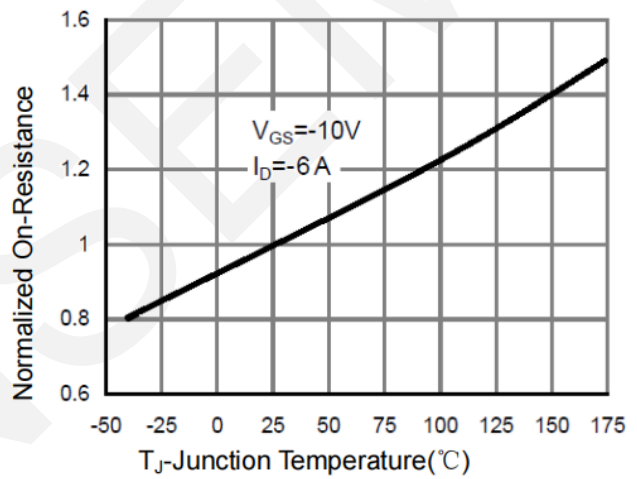
Rdson-Junction Temperature
