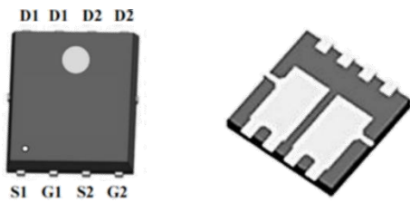
PDFN5x6 Pin Description
