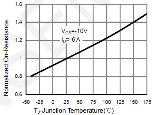
Rdson-Junction Temperature
