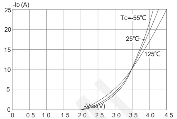
Transfer Characteristics
