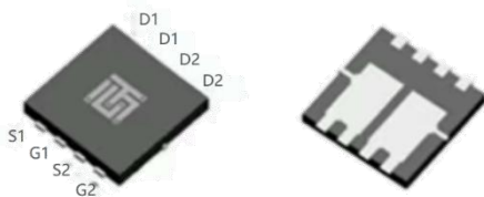
PDFN3x3 Pin Description
