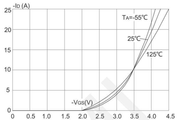
Transfer Characteristics
