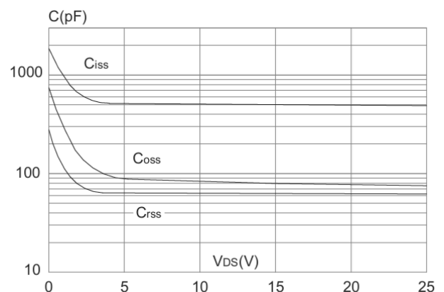
Capacitance Characteristics
