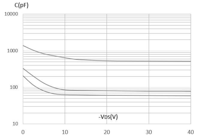
Capacitance Characteristics
