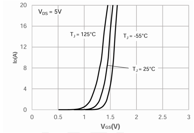
Transfer Characteristics
