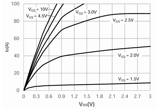
Output Characteristics
