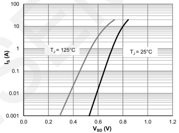
Body-Diode Characteristics
