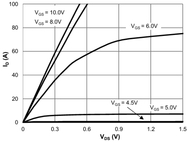
Saturation Characteristics
