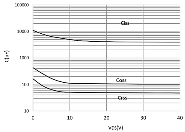
Capacitance Characteristics
