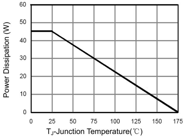
Power De-rating
