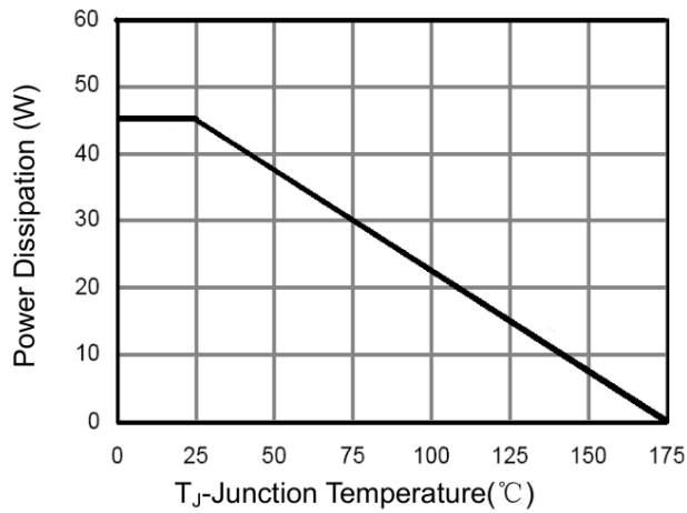
Power De-rating
