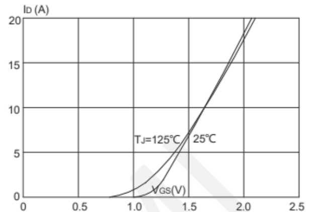
Figure 2 Transfer Characteristics
