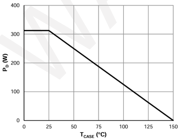
Power De-rating
