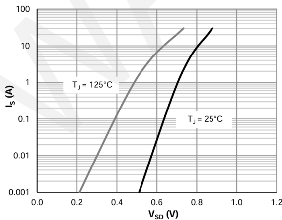
Body-Diode Characteristics
