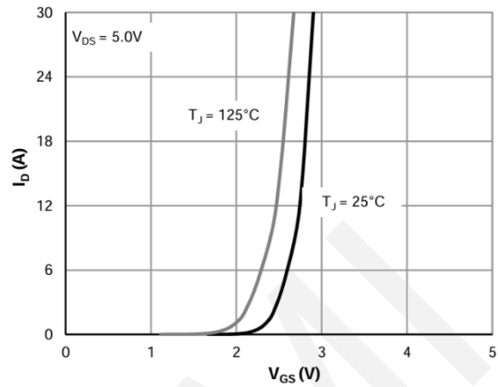
Transfer Characteristics
