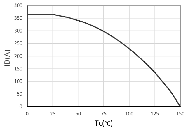
Current De-rating
