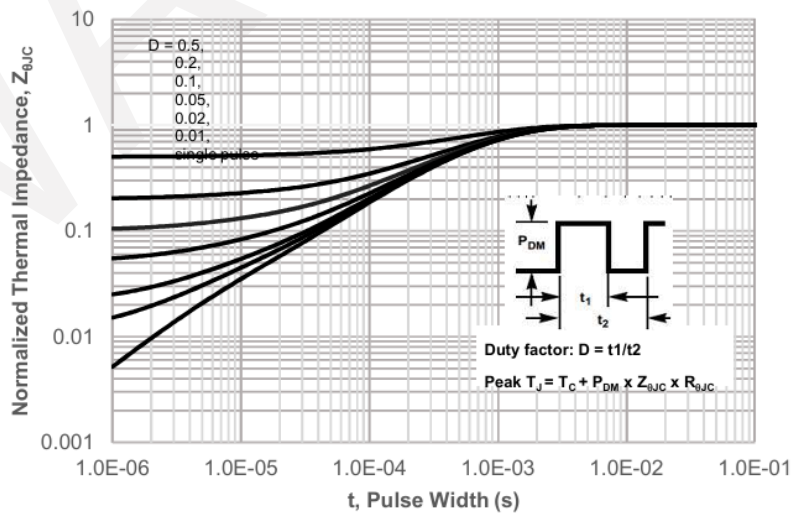
Normalized Maximum Transient Thermal Impedance
