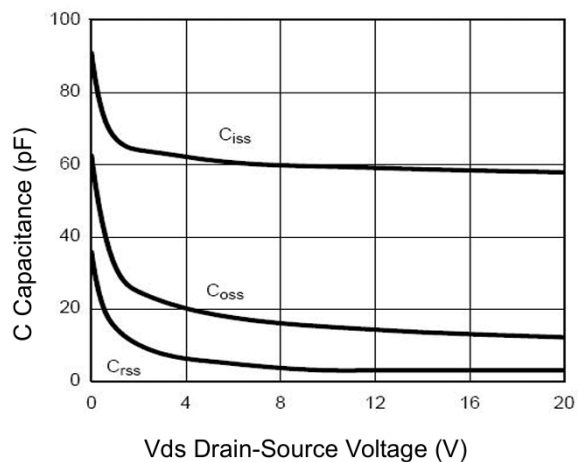
Capacitance Characteristics
