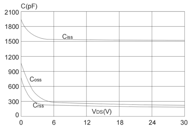
Capacitance Characteristics
