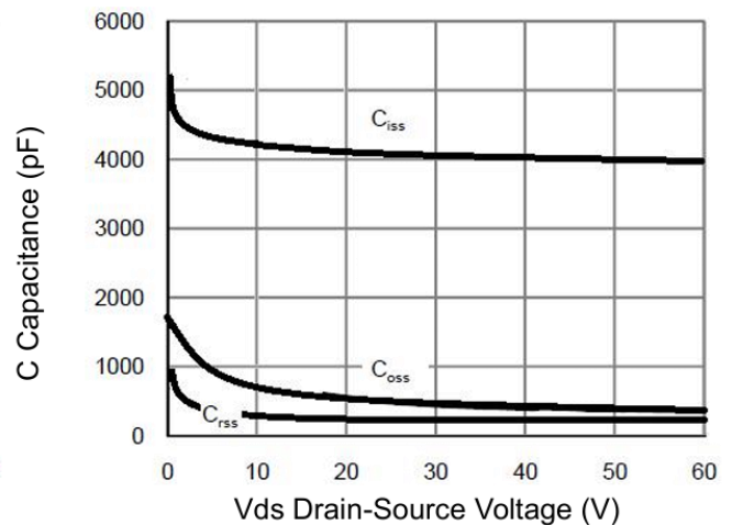
Capacitance Characteristics
