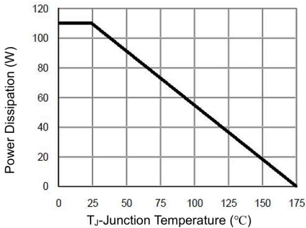
Power De-rating
