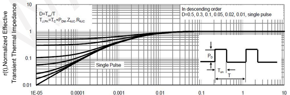
Square Wave Pulse Duration(sec) Maximum Effective Transient Thermal Impedance, Junction-to-Case
