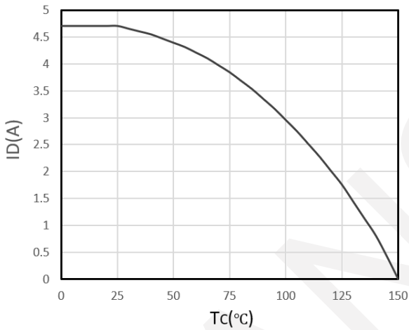
Drain current
