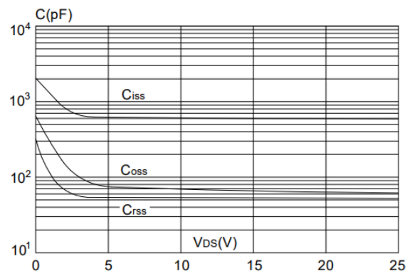
Capacitance Characteristics
