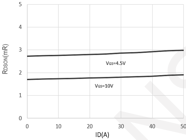
Rdson-Drain Current
