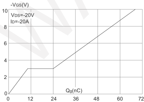
Gate Charge
