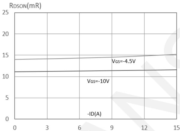
Rdson-Drain Current
