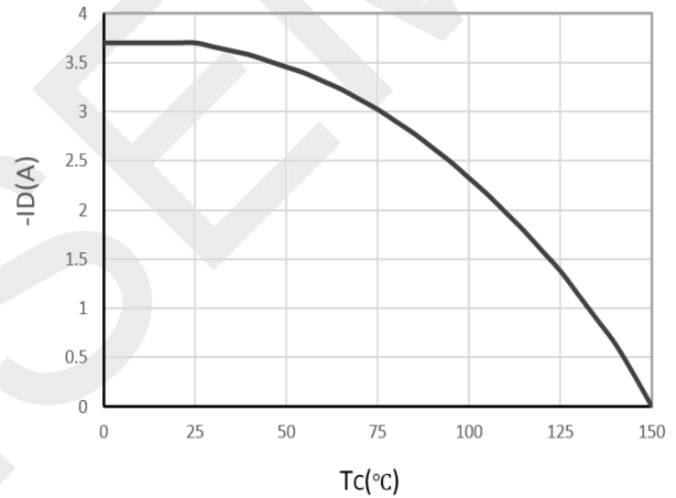
Current De-rating
