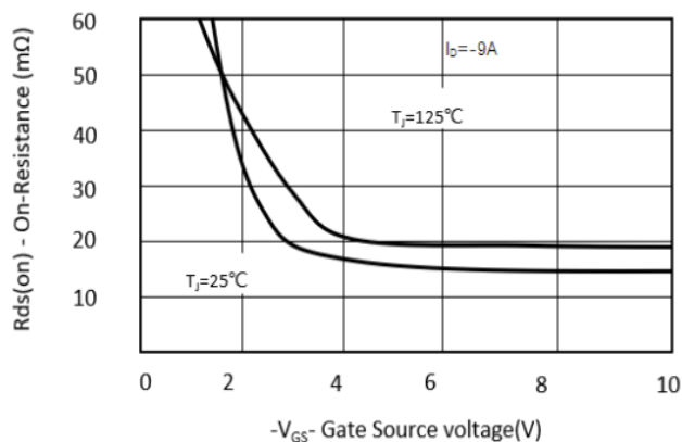
On-Resistance Vs. Gate-Source Voltage
