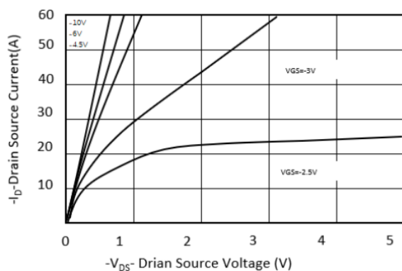
Output Characteristics
